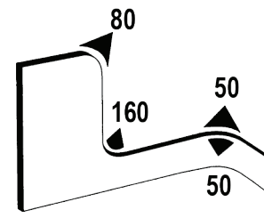
Bend Radius
